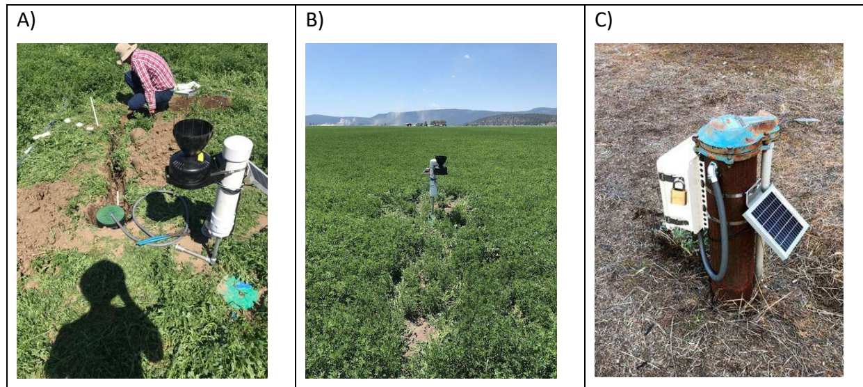
Figure 2: Field stations in Siskiyou County with various sensor configurations.
