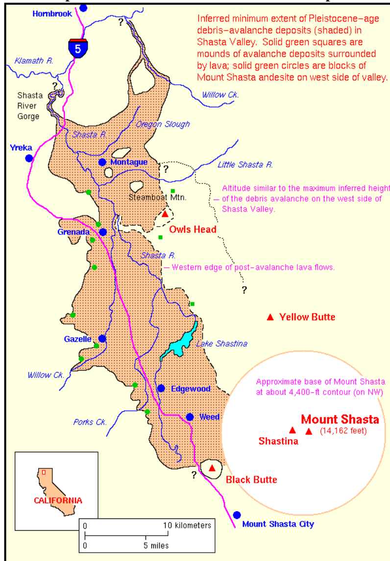
Map 107: Mount Shasta Debris Avalanche Deposit
